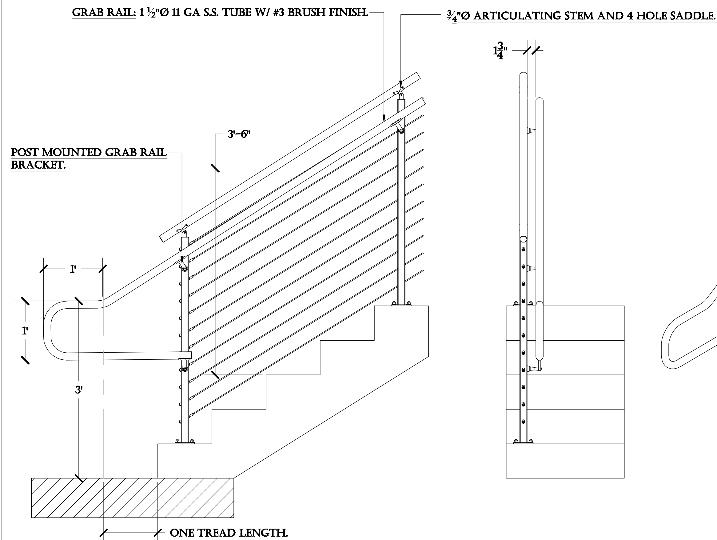
SPI-2000 42" STAIR GUARD RAILING.
