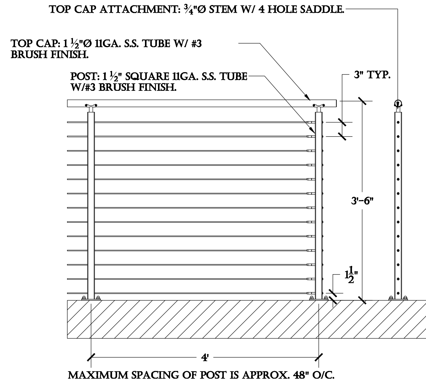
SPI-2000 LEVEL 42" GUARD RAILING.
