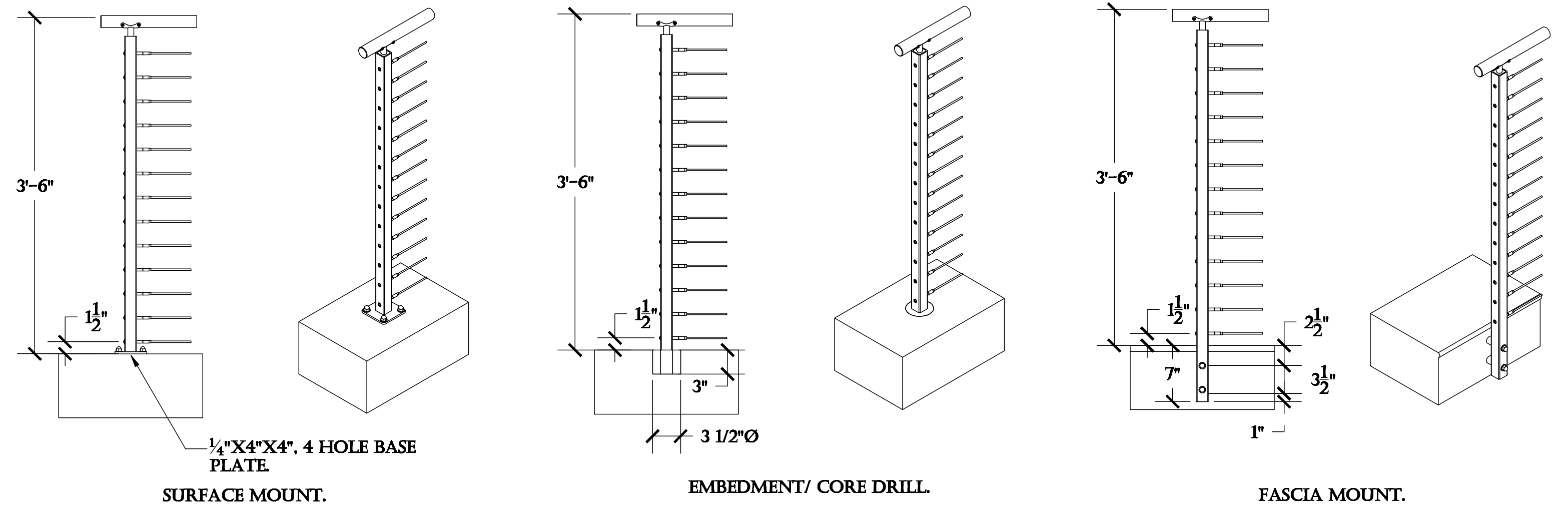
SPI-2000 TYPICAL MOUNTING OPTIONS.
